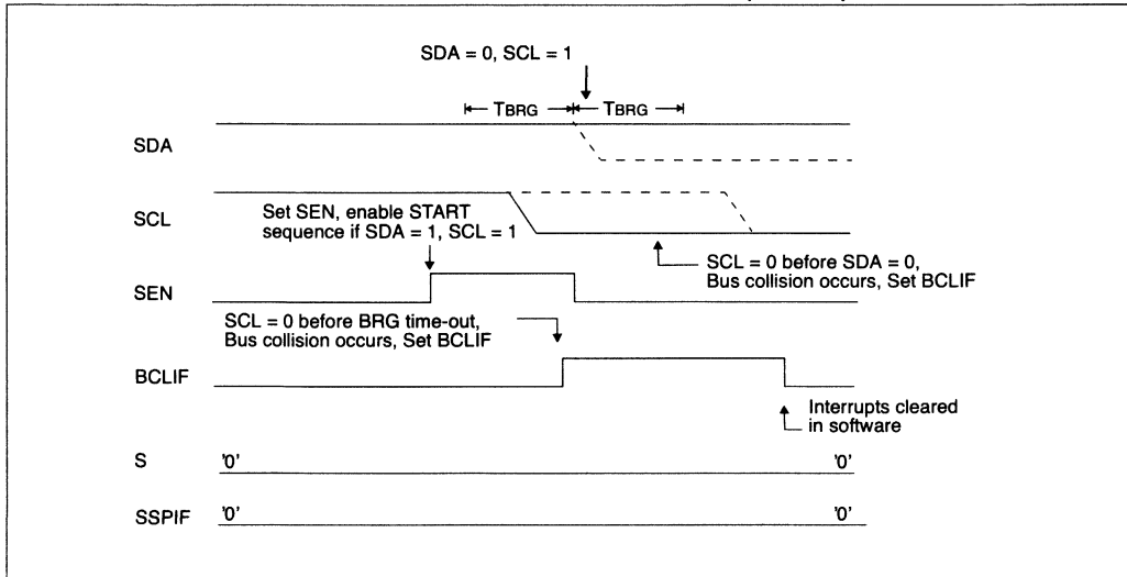
FIGURE 9-21: BUS COLLISION DURING START CONDITION (SCL = 0)
