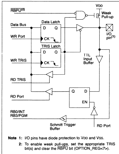
FIGURE 3-3: BLOCK DIAGRAM OF RB3:RB0 PINS
