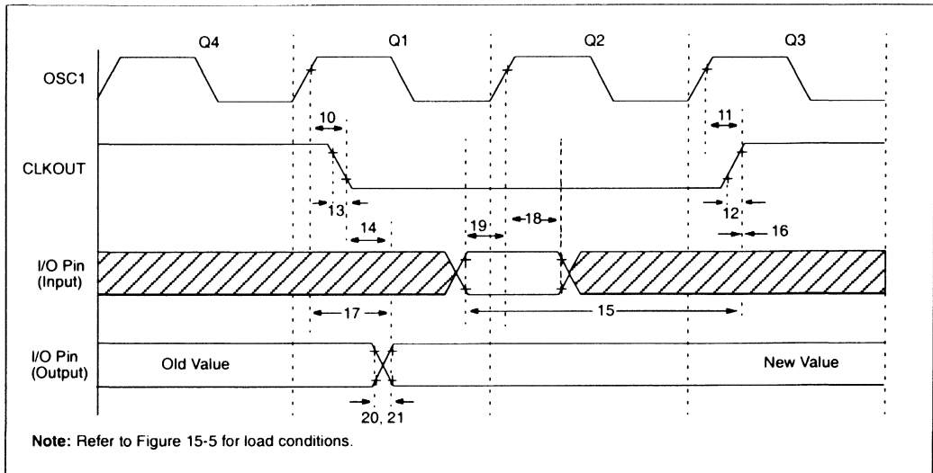
FIGURE 15-7: CLKOUT AND I/O TIMING
