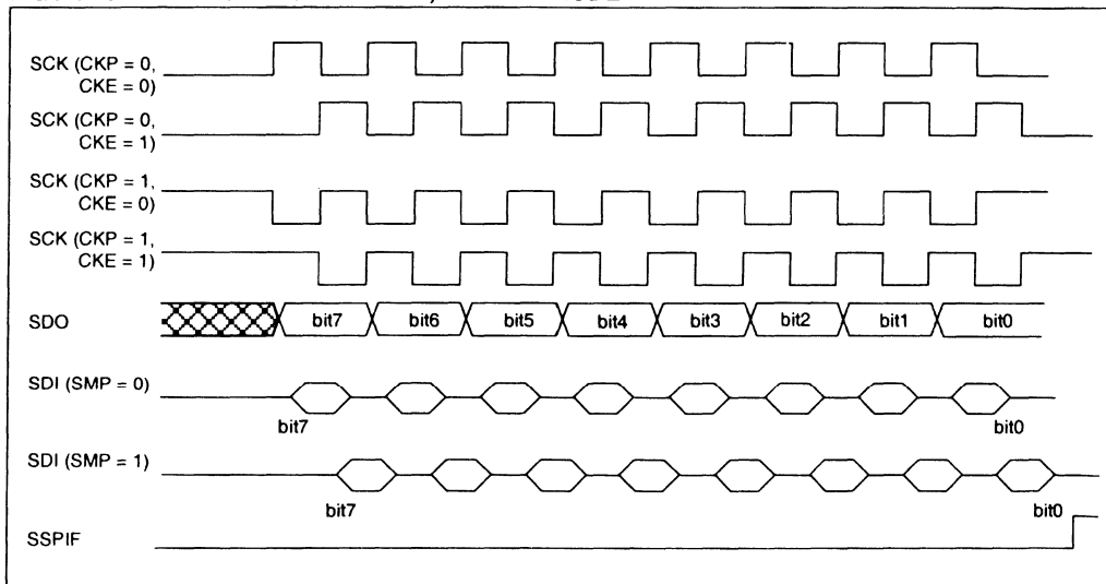
FIGURE 9-2: SPI MODE TIMING, MASTER MODE
