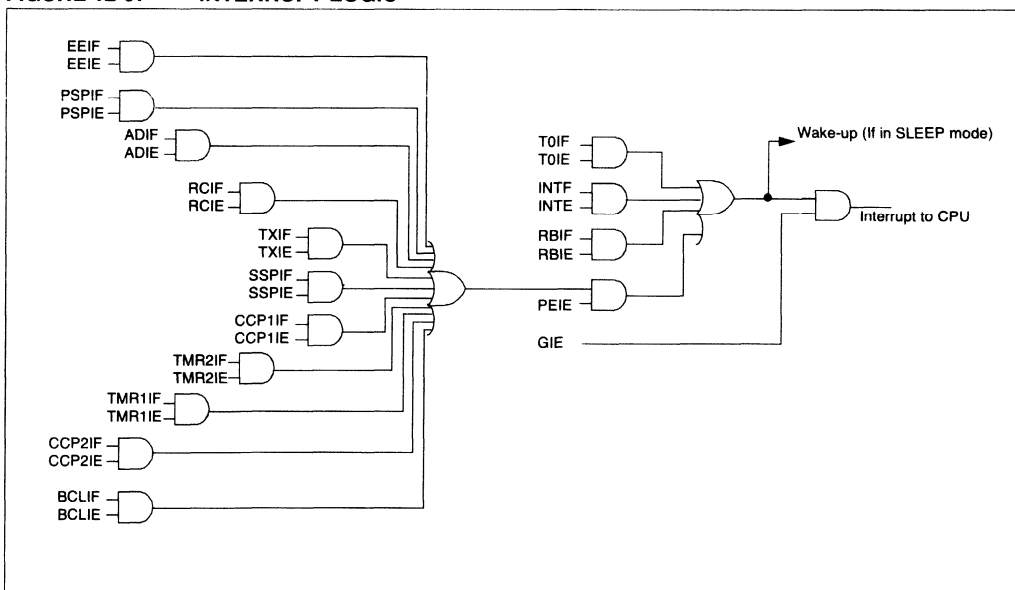
FIGURE 12-9: INTERRUPT LOGIC
