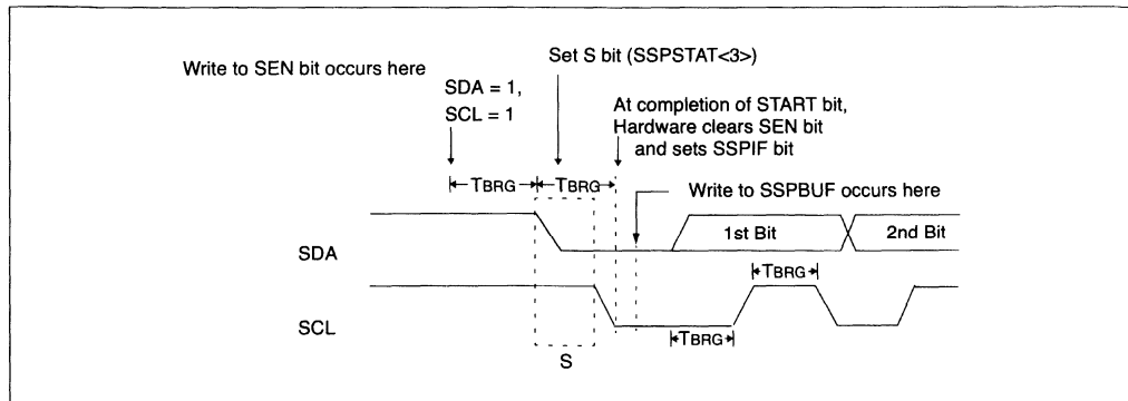
FIGURE 9-12: FIRST START BIT TIMING
