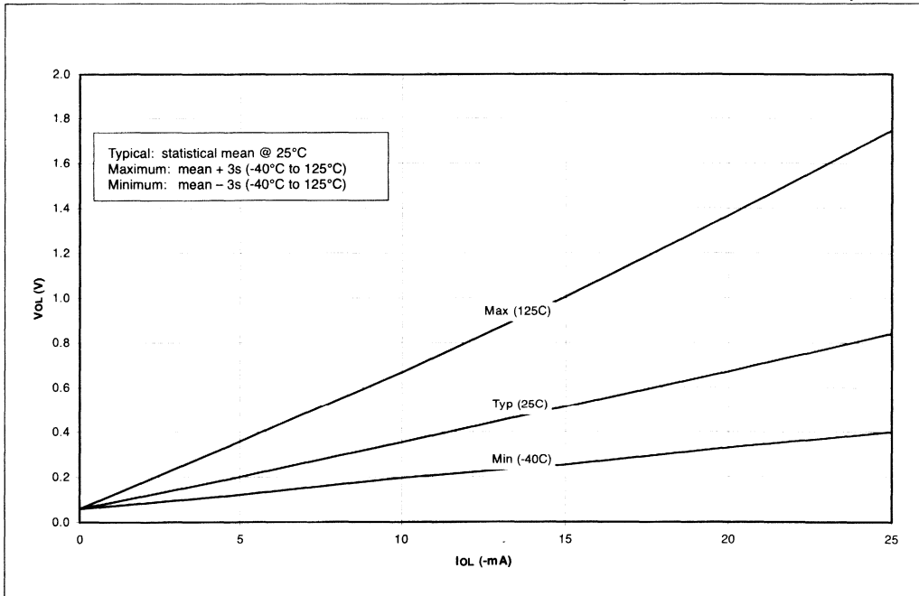
FIGURE 16-18: TYPICAL, MINIMUM AND MAXIMUM VOL vs. IOL (VDD=5V, -40°C TO 125°C)
