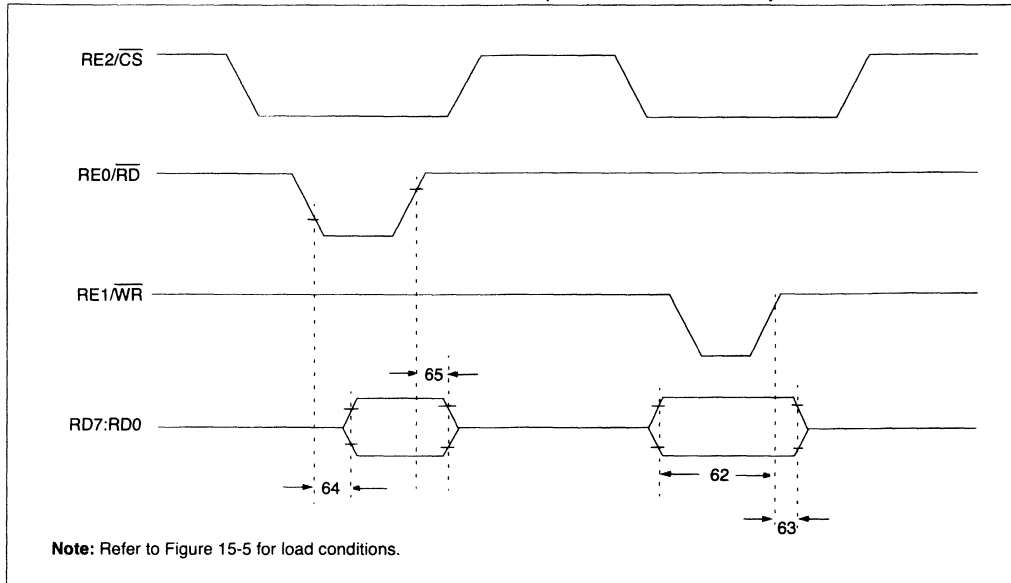
FIGURE 15-12: PARALLEL SLAVE PORT TIMING (PIC16F874/877 ONLY)
