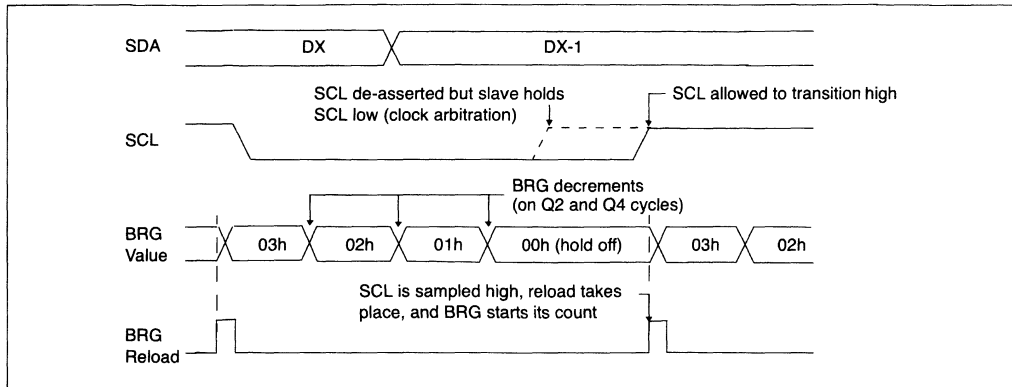
FIGURE 9-11: BAUD RATE GENERATOR TIMING WITH CLOCK ARBITRATION
