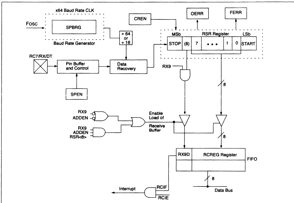
FIGURE 10-6: USART RECEIVE BLOCK DIAGRAM
