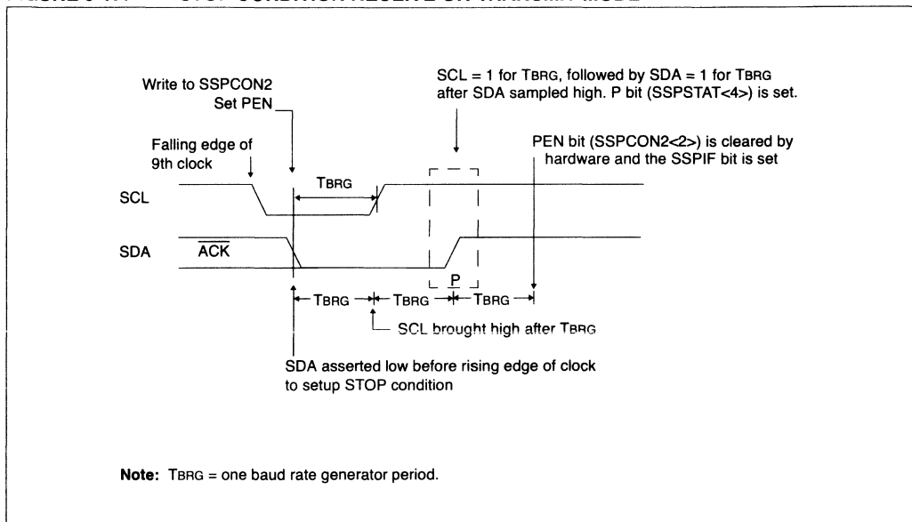
FIGURE 9-17: STOP CONDITION RECEIVE OR TRANSMIT MODE
