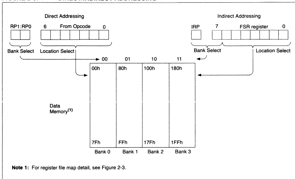
FIGURE 2-6: DIRECT/INDIRECT ADDRESSING
