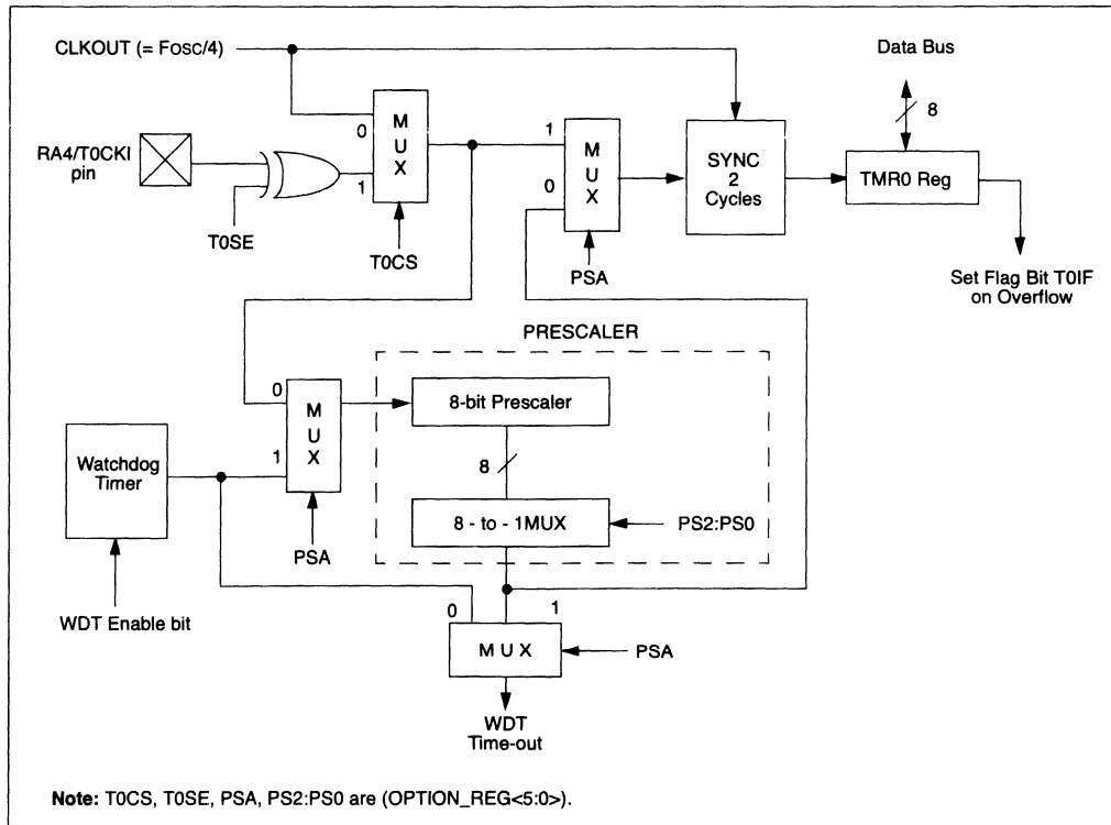
FIGURE 5-1: BLOCK DIAGRAM OF THE TIMER0/WDT PRESCALER
