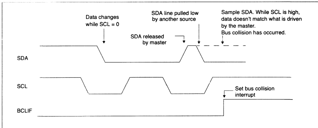
FIGURE 9-19: BUS COLLISION TIMING FOR TRANSMIT AND ACKNOWLEDGE
