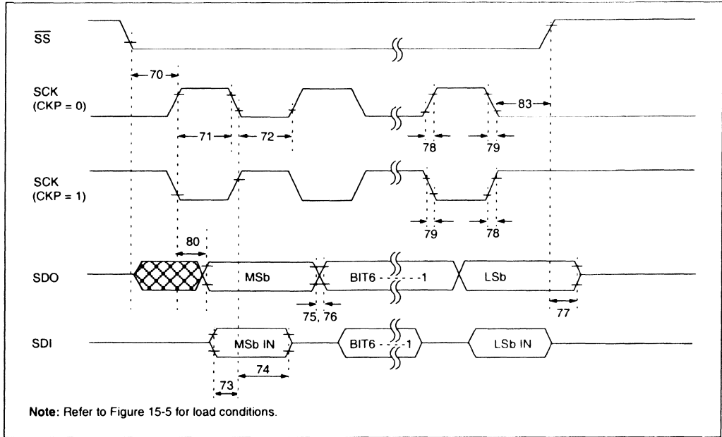
FIGURE 15-15: SPI SLAVE MODE TIMING (CKE = 0)
