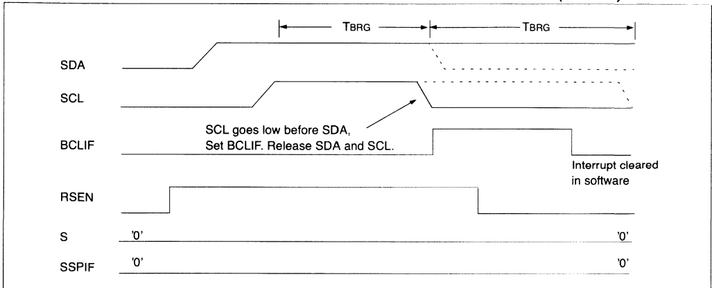
FIGURE 9-24: BUS COLLISION DURING REPEATED START CONDITION (CASE 2)
