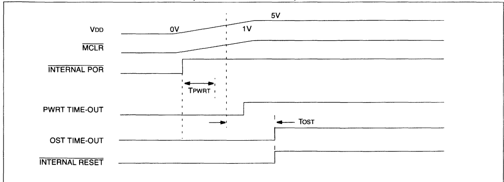
FIGURE 12-8: SLOW RISE TIME ( \overline{\text{MCLR}} TIED TO V_{\text{DD}} )
