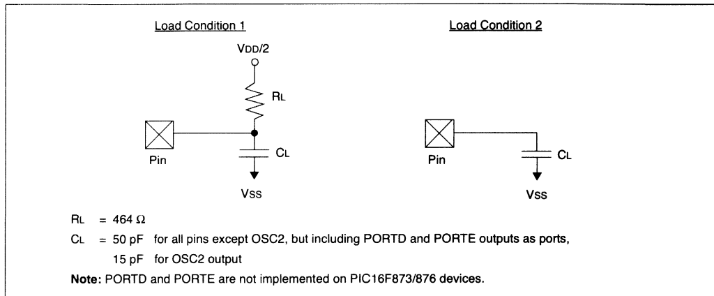
FIGURE 15-5: LOAD CONDITIONS
