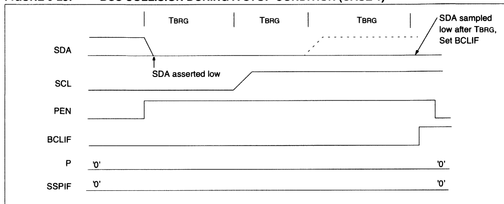
FIGURE 9-25: BUS COLLISION DURING A STOP CONDITION (CASE 1)
