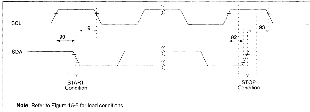
FIGURE 15-17: I 2 C BUS START/STOP BITS TIMING
