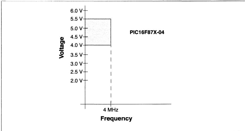
FIGURE 15-3: PIC16F87X-04 VOLTAGE-FREQUENCY GRAPH (ALL TEMPERATURE RANGES)
