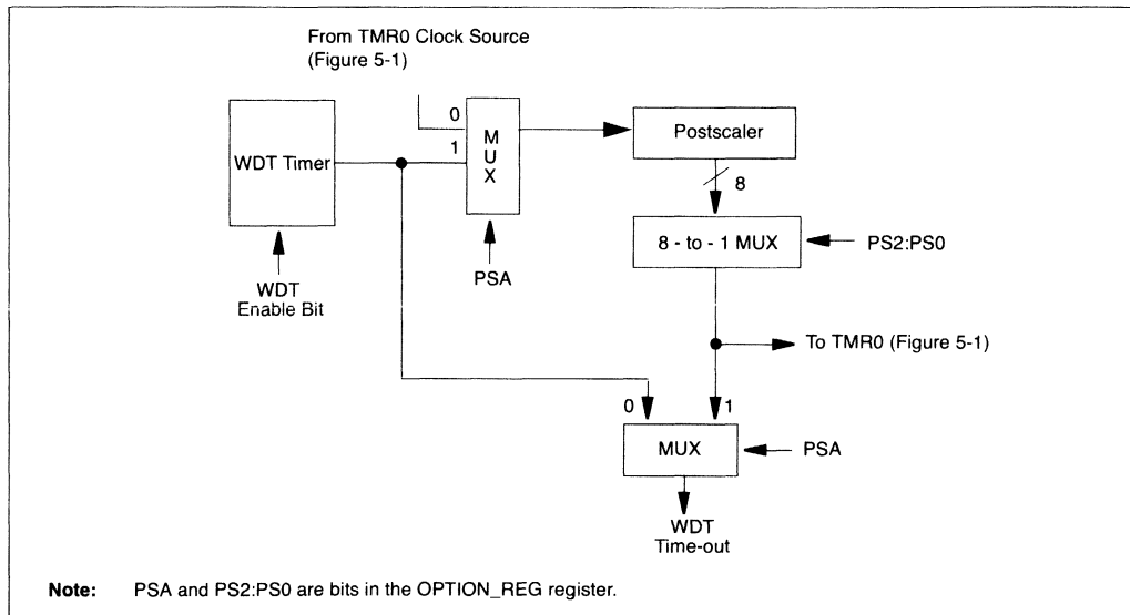
FIGURE 12-10: WATCHDOG TIMER BLOCK DIAGRAM
