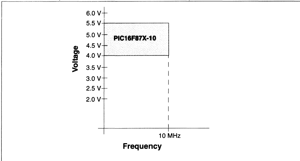
FIGURE 15-4: PIC16F87X-10 VOLTAGE-FREQUENCY GRAPH (EXTENDED TEMPERATURE RANGE ONLY)
