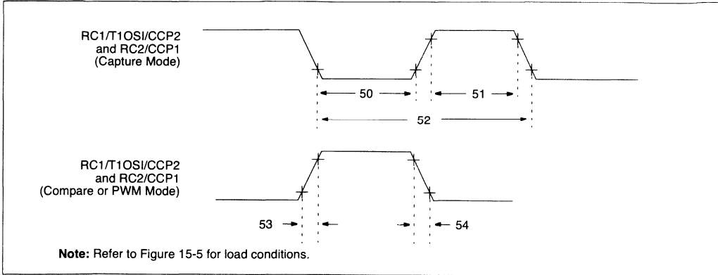
FIGURE 15-11: CAPTURE/COMPARE/PWM TIMINGS (CCP1 AND CCP2)
