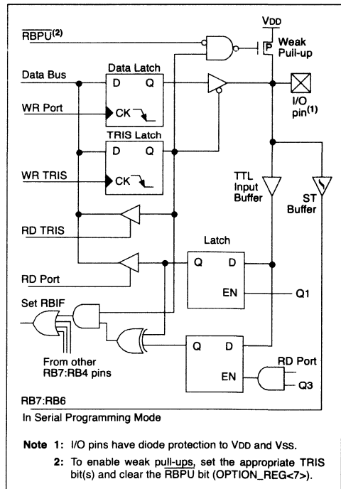
FIGURE 3-4: BLOCK DIAGRAM OF RB7:RB4 PINS
