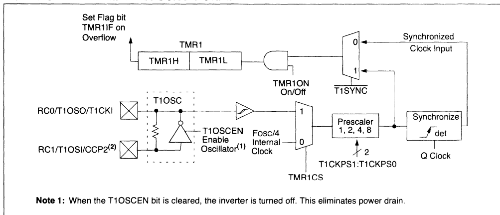
FIGURE 6-2: TIMER1 BLOCK DIAGRAM
