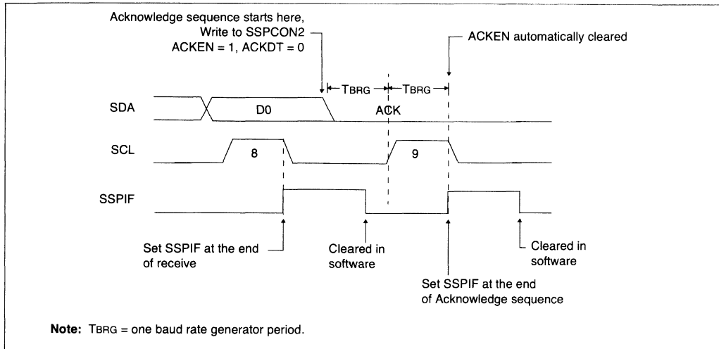
FIGURE 9-16: ACKNOWLEDGE SEQUENCE WAVEFORM
