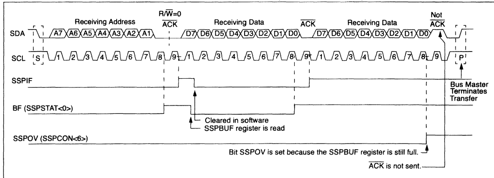
FIGURE 9-6: I 2 C WAVEFORMS FOR RECEPTION (7-BIT ADDRESS)
