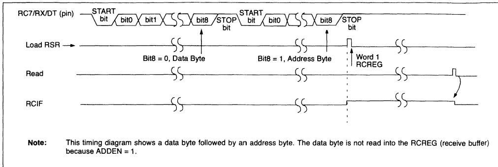
FIGURE 10-7: ASYNCHRONOUS RECEPTION WITH ADDRESS DETECT
