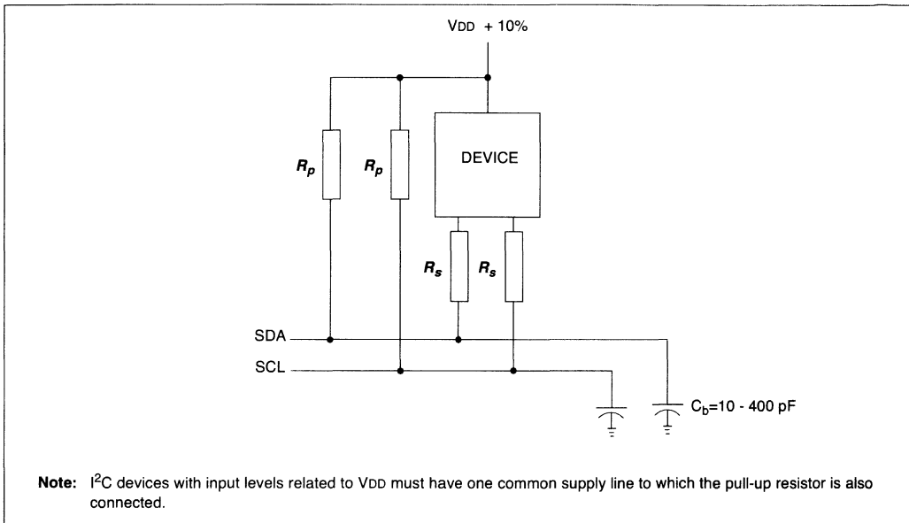
FIGURE 9-27: SAMPLE DEVICE CONFIGURATION FOR I 2 C BUS
