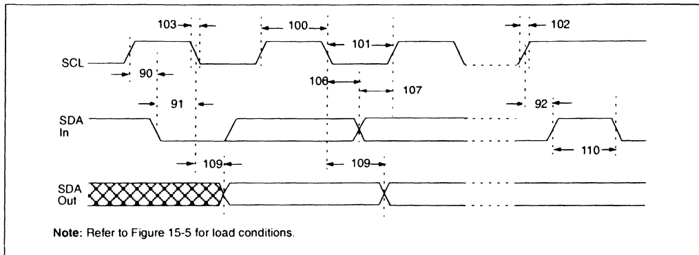
FIGURE 15-18: I 2 C BUS DATA TIMING
