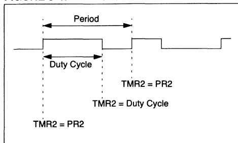
FIGURE 8-4: PWM OUTPUT
