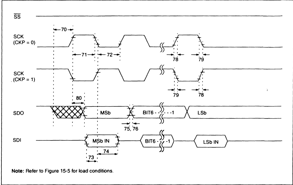
FIGURE 15-13: SPI MASTER MODE TIMING (CKE = 0, SMP = 0)
