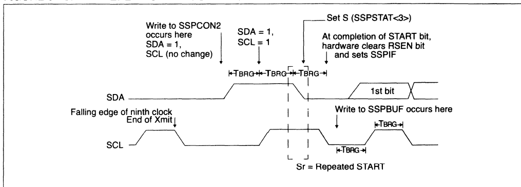
FIGURE 9-13: REPEAT START CONDITION WAVEFORM
