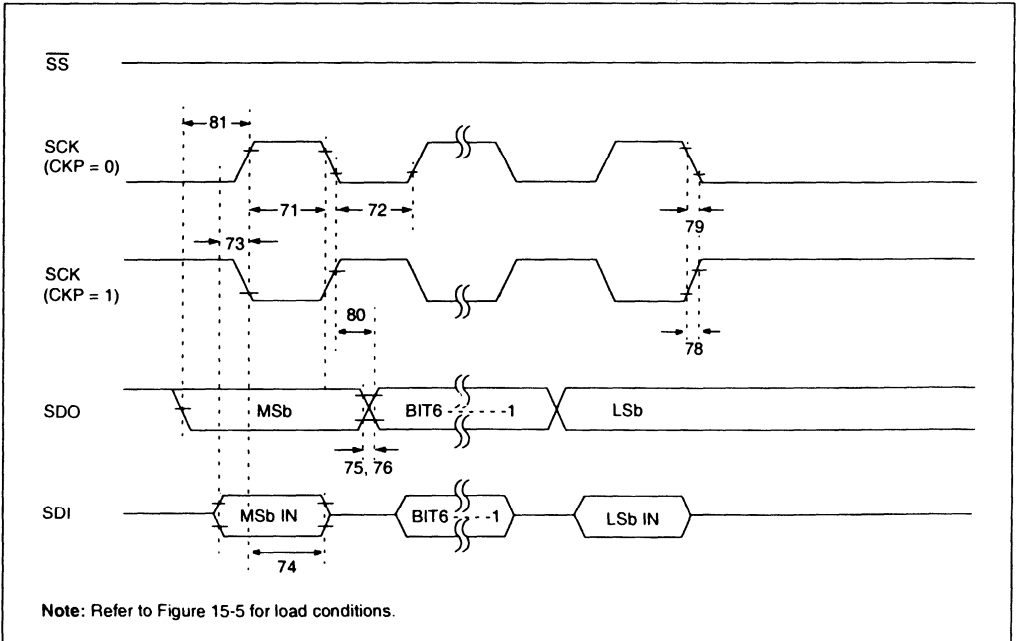
FIGURE 15-14: SPI MASTER MODE TIMING (CKE = 1, SMP = 1)
