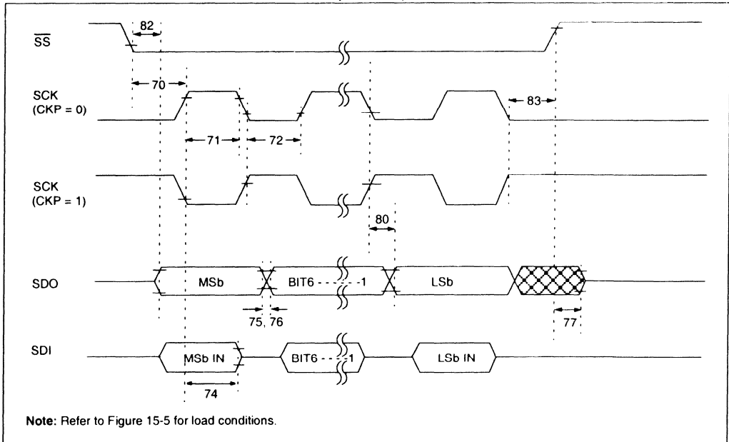
FIGURE 15-16: SPI SLAVE MODE TIMING (CKE = 1)
