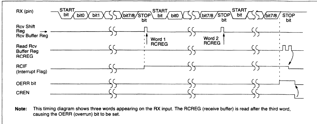
FIGURE 10-5: ASYNCHRONOUS RECEPTION
