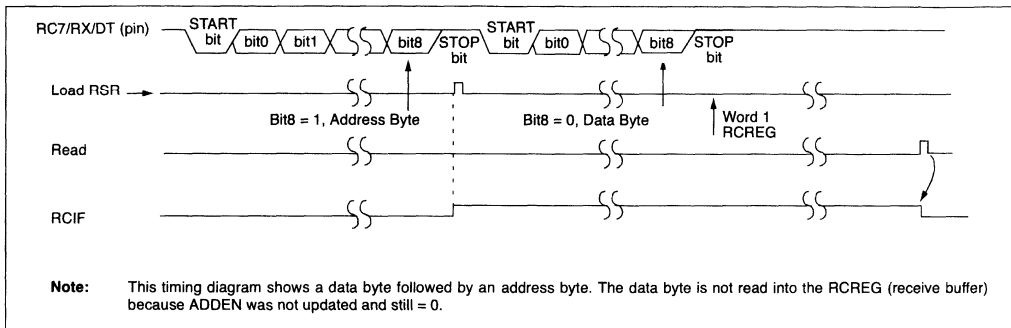
FIGURE 10-8: ASYNCHRONOUS RECEPTION WITH ADDRESS BYTE FIRST
