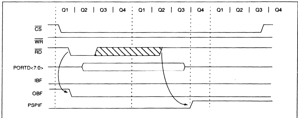
FIGURE 3-11: PARALLEL SLAVE PORT READ WAVEFORMS
