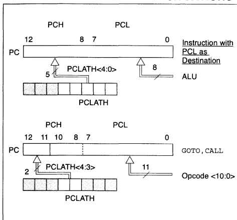
FIGURE 2-5: LOADING OF PC IN DIFFERENT SITUATIONS
