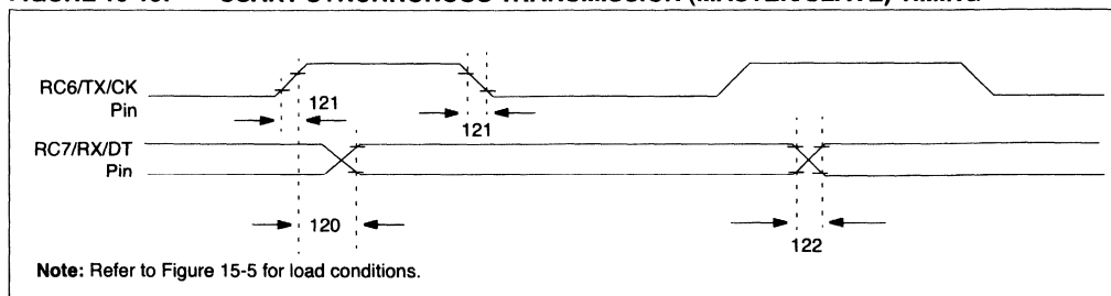
FIGURE 15-19: USART SYNCHRONOUS TRANSMISSION (MASTER/SLAVE) TIMING
