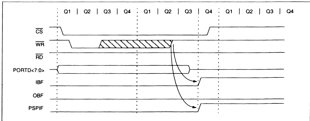
FIGURE 3-10: PARALLEL SLAVE PORT WRITE WAVEFORMS
