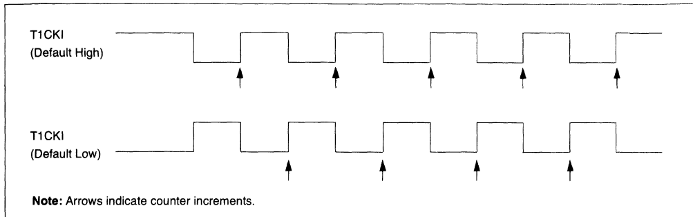
FIGURE 6-1: TIMER1 INCREMENTING EDGE
