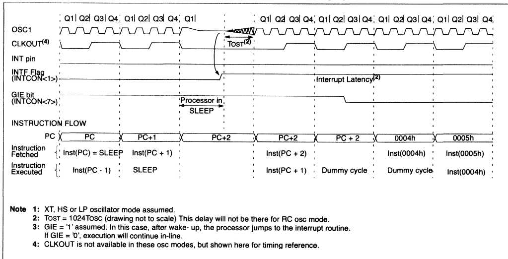
FIGURE 12-11: WAKE-UP FROM SLEEP THROUGH INTERRUPT
