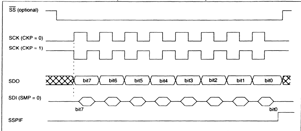
FIGURE 9-3: SPI MODE TIMING (SLAVE MODE WITH CKE = 0)
