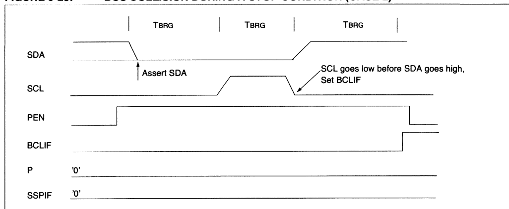
FIGURE 9-26: BUS COLLISION DURING A STOP CONDITION (CASE 2)
