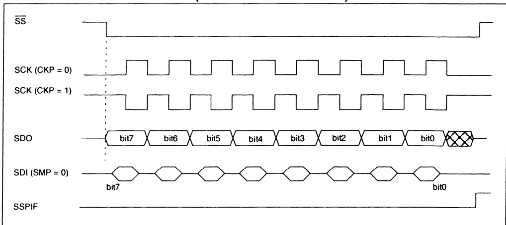
FIGURE 9-4: SPI MODE TIMING (SLAVE MODE WITH CKE = 1)
