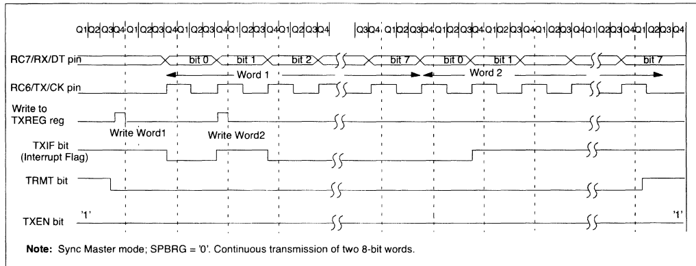
FIGURE 10-9: SYNCHRONOUS TRANSMISSION
