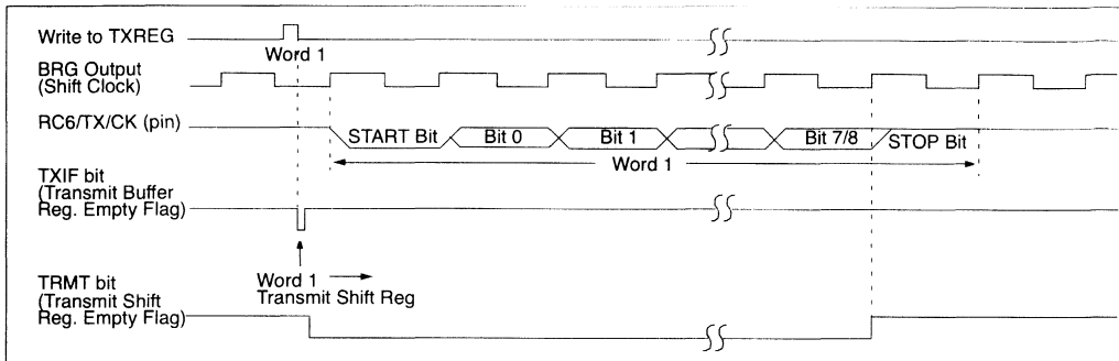
FIGURE 10-3: ASYNCHRONOUS MASTER TRANSMISSION (BACK TO BACK)
