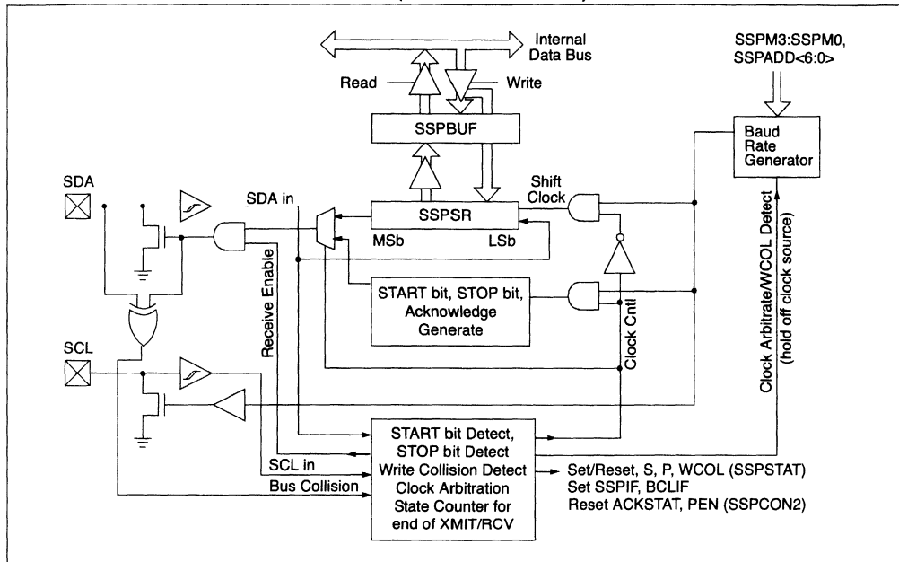
FIGURE 9-9: SSP BLOCK DIAGRAM (I 2 C MASTER MODE)
