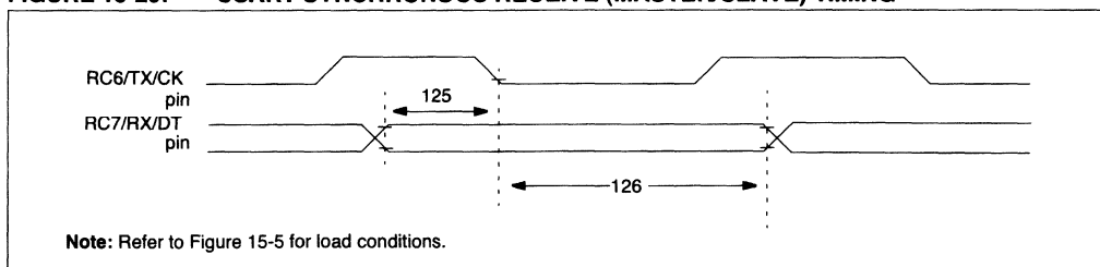
FIGURE 15-20: USART SYNCHRONOUS RECEIVE (MASTER/SLAVE) TIMING
