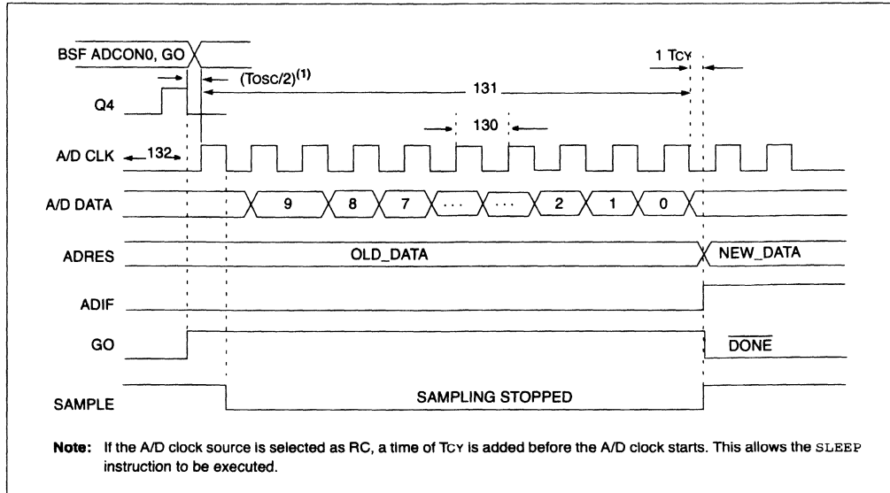
FIGURE 15-21: A/D CONVERSION TIMING
