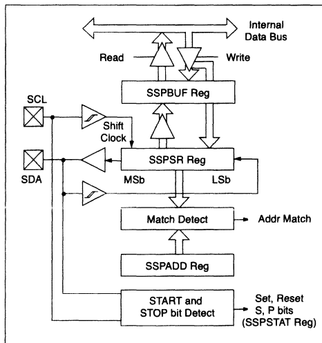
FIGURE 9-5: I 2 C SLAVE MODE BLOCK DIAGRAM
