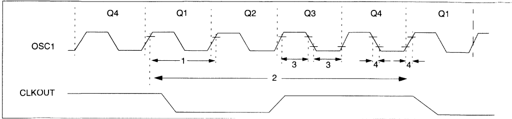
FIGURE 15-6: EXTERNAL CLOCK TIMING
