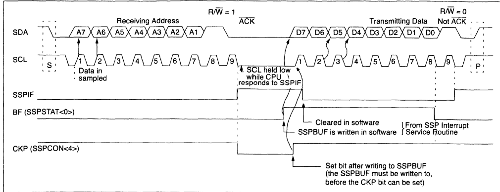
FIGURE 9-7: I 2 C WAVEFORMS FOR TRANSMISSION (7-BIT ADDRESS)
