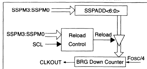
FIGURE 9-10: BAUD RATE GENERATOR BLOCK DIAGRAM
