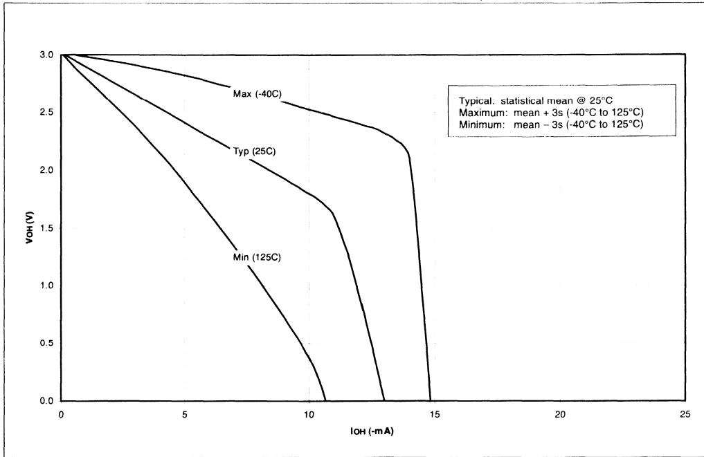
FIGURE 16-17: TYPICAL, MINIMUM AND MAXIMUM VOH vs. IOH (VDD=3V, -40°C TO 125°C)
