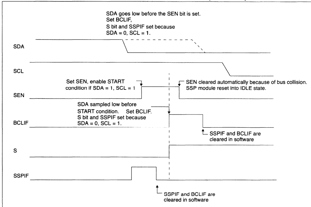
FIGURE 9-20: BUS COLLISION DURING START CONDITION (SDA ONLY)
