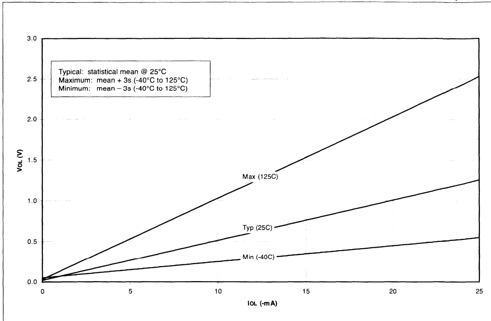
FIGURE 16-19: TYPICAL, MINIMUM AND MAXIMUM VOL vs. IOL (VDD=3V, -40°C TO 125°C)
