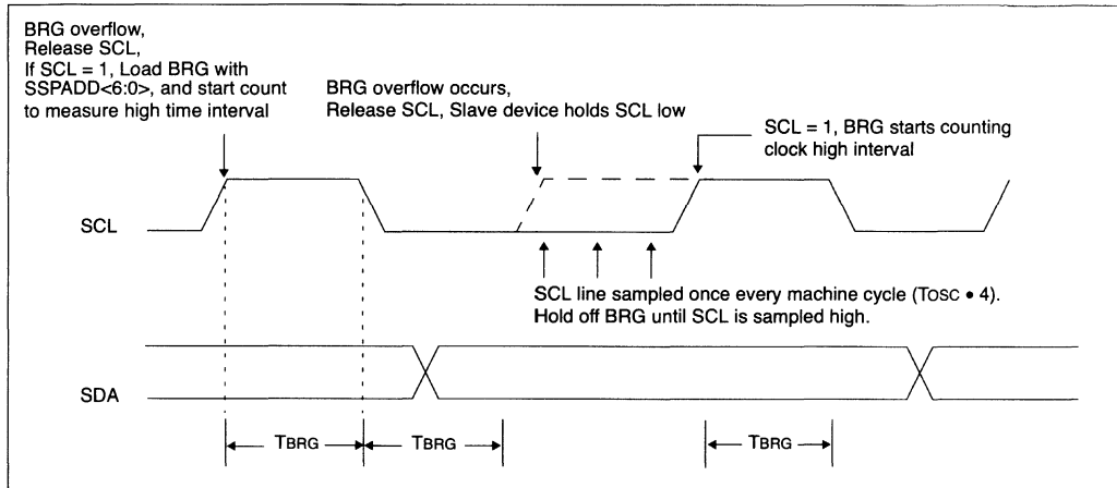
FIGURE 9-18: CLOCK ARBITRATION TIMING IN MASTER TRANSMIT MODE
