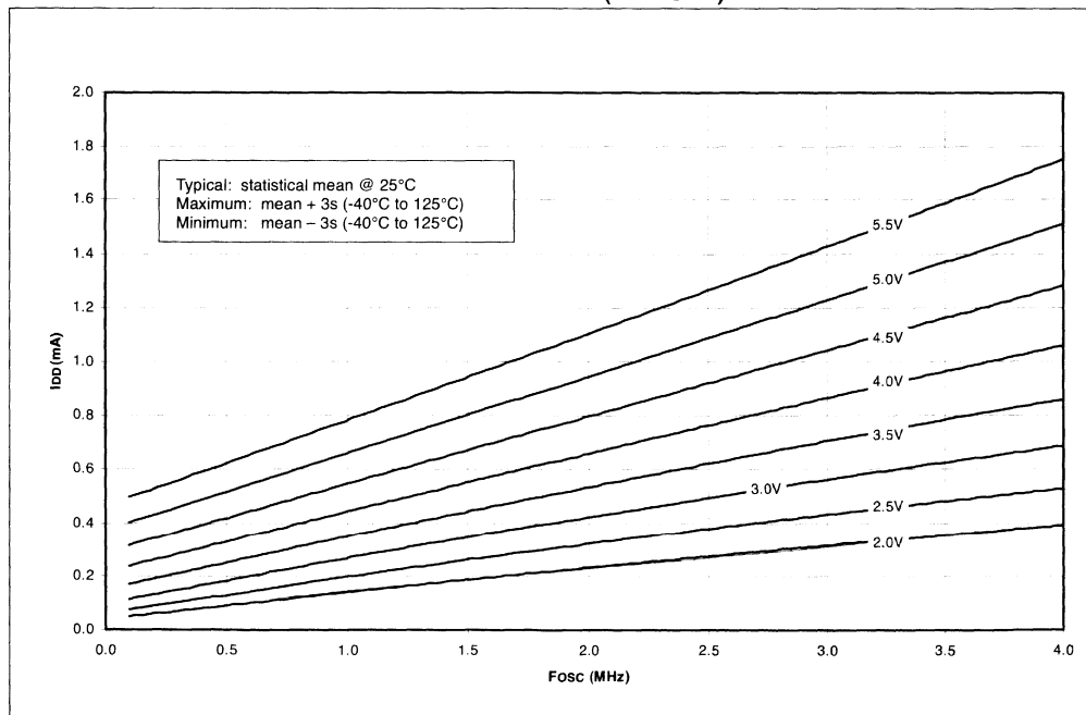
FIGURE 16-4: MAXIMUM I_{DD} vs. Fosc OVER V_{DD} (LP MODE)
